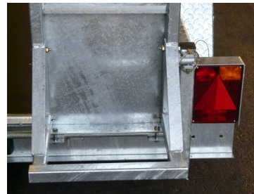
Ramp Support - Protected Plug-In Light Clusters - Bolt On Lashing Links
